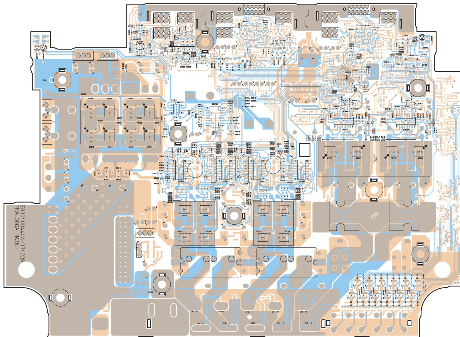
MAIN P.W.Board (Foil Side View)
