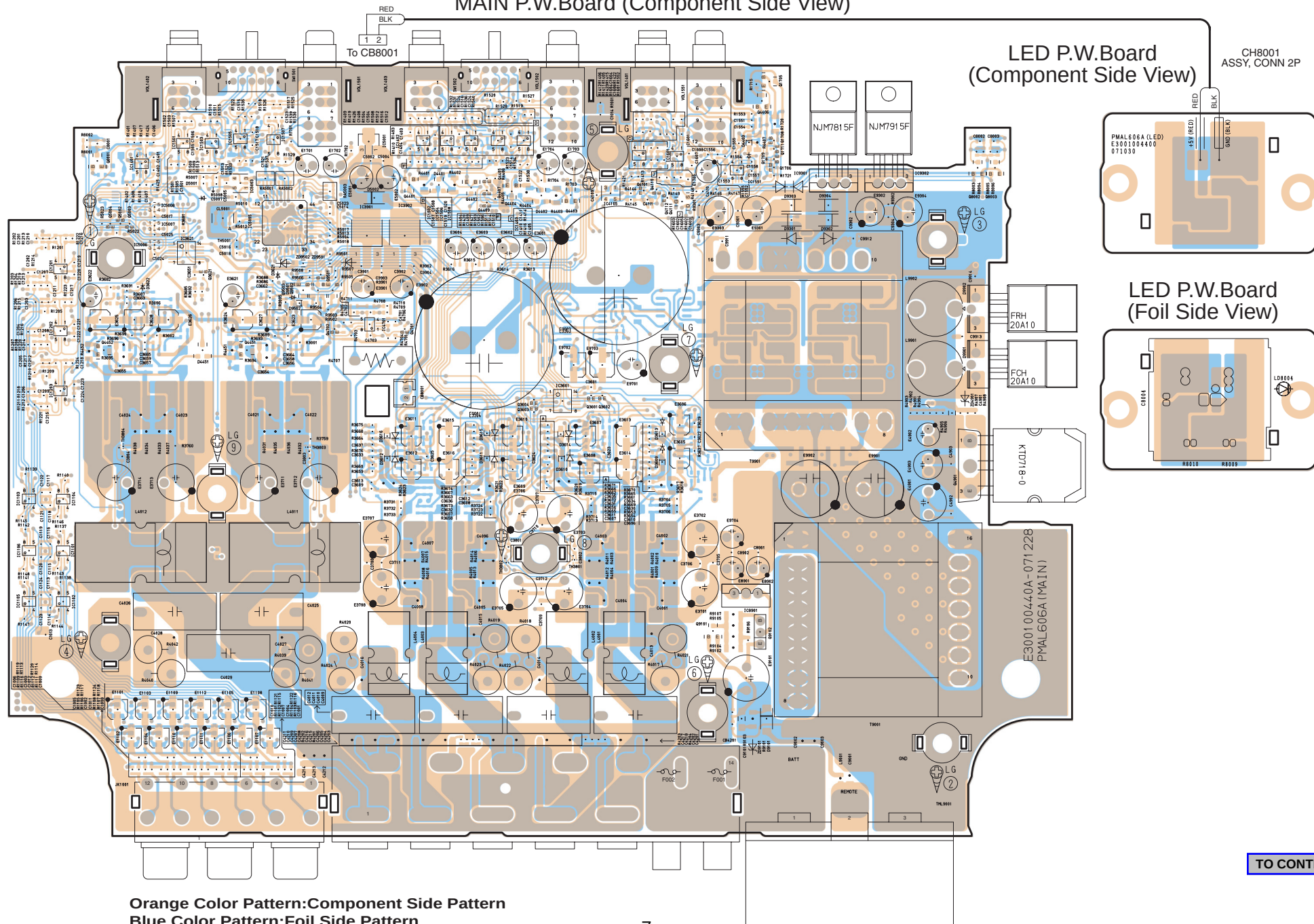
MAIN P.W.Board (Component Side View)
